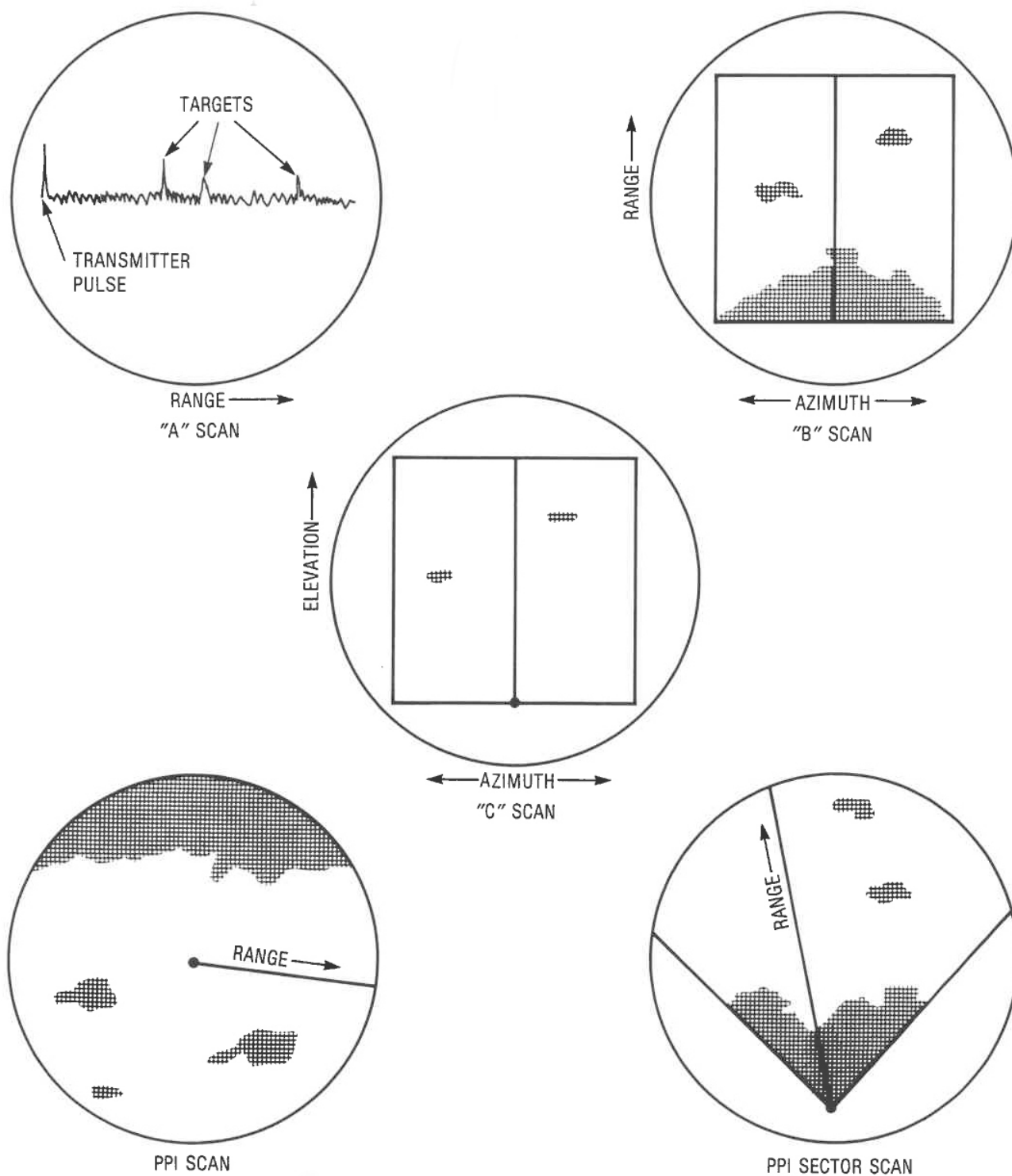
Figure 40. Various radar indicator presentations.
