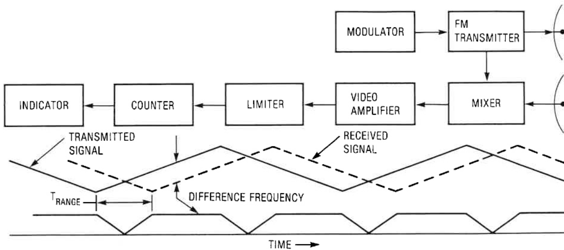
Figure 13. FM-CW range measuring radar block diagram.
